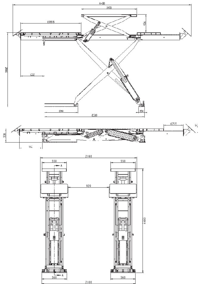
Figure 2-Lift Dimensions
